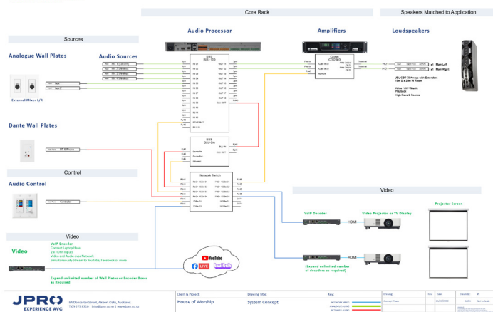
HOUSE OF WORSHIP JBL Audio System (15m)
